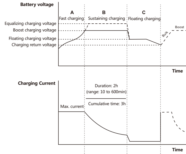
Fig. 1-5 Battery charging stages diagram
